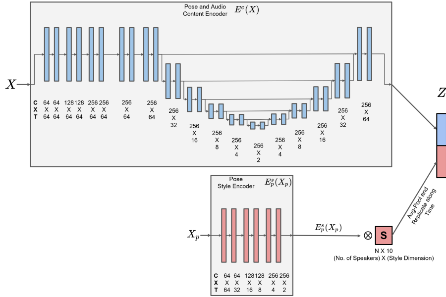
Fig. 10: Encoder Architecture
